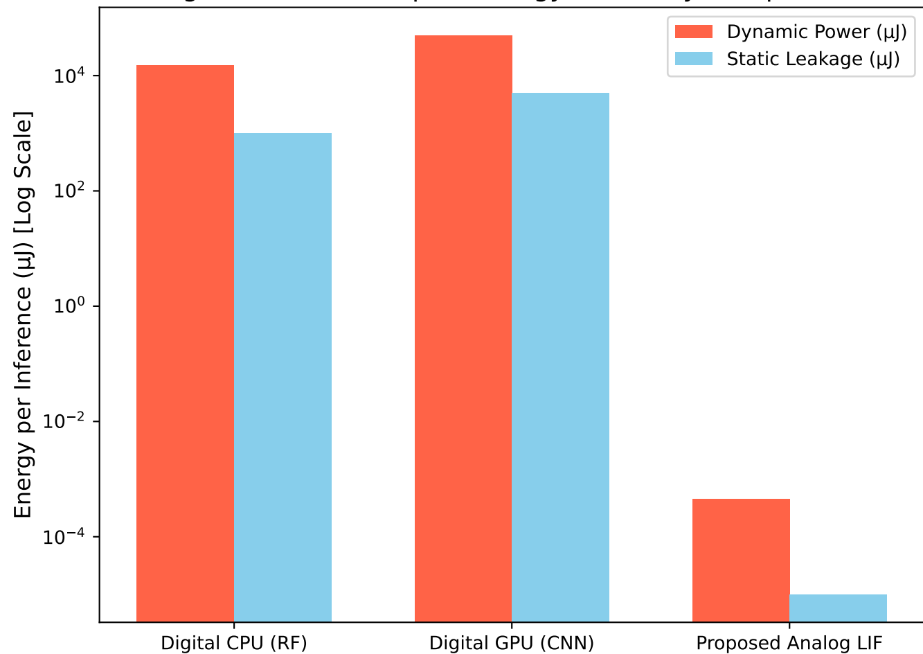
Figure 5: Neuromorphic Energy Efficiency Comparison
